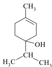
II terpinen-4-ol
