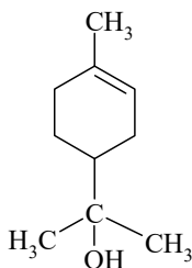
III terpineol
